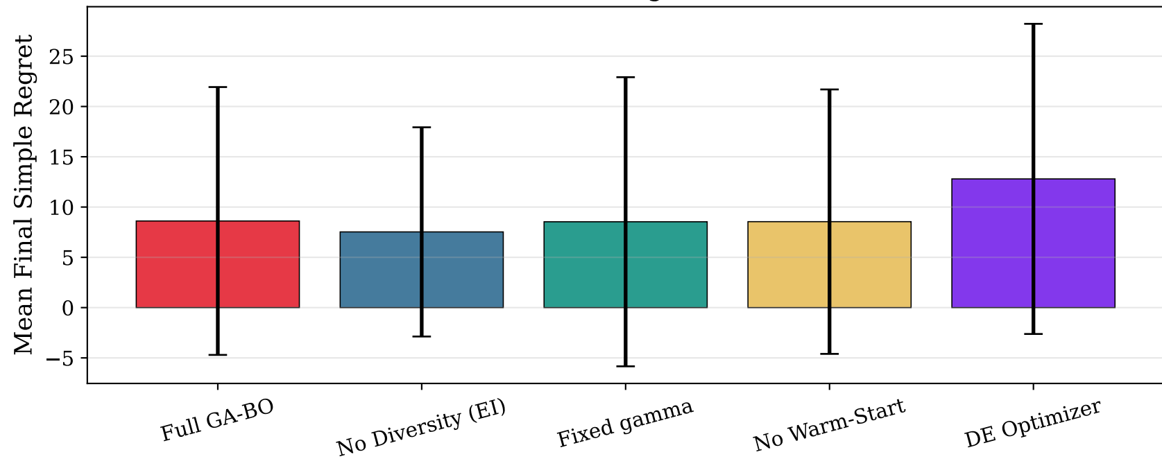
Ablation: Mean Final Regret (lower = better)
